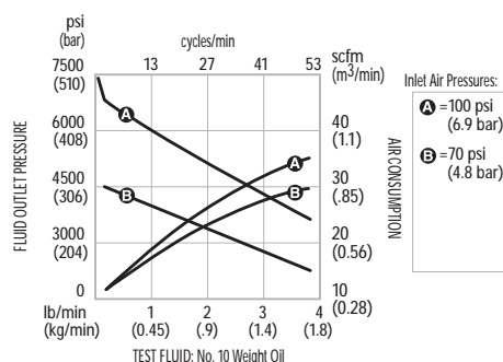
Pump Performance
